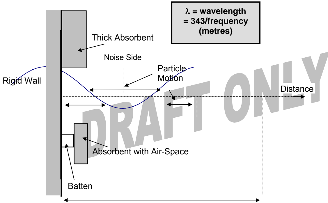
Figure 1 – An Application of Acoustic Absorbent
